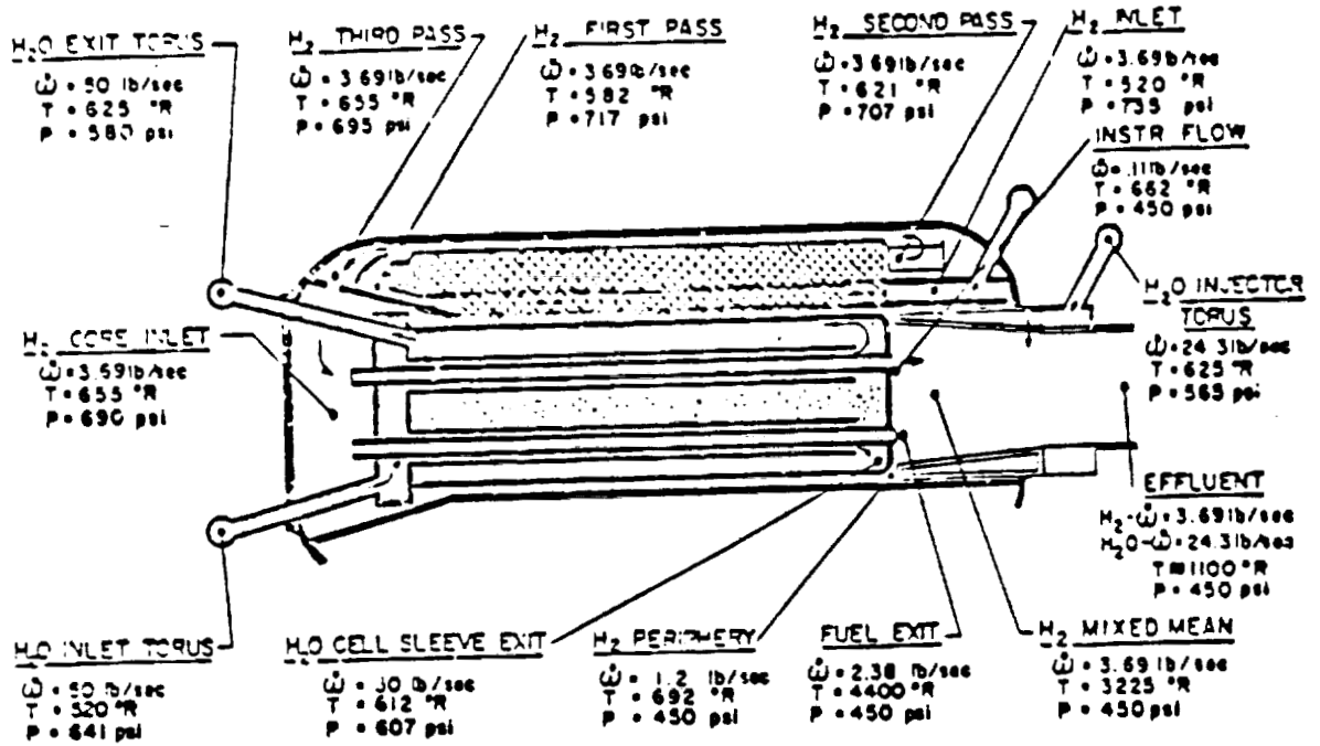
FIGURE 42. NUCLEAR FURNACE STATE POINT SCHEMATIC.
