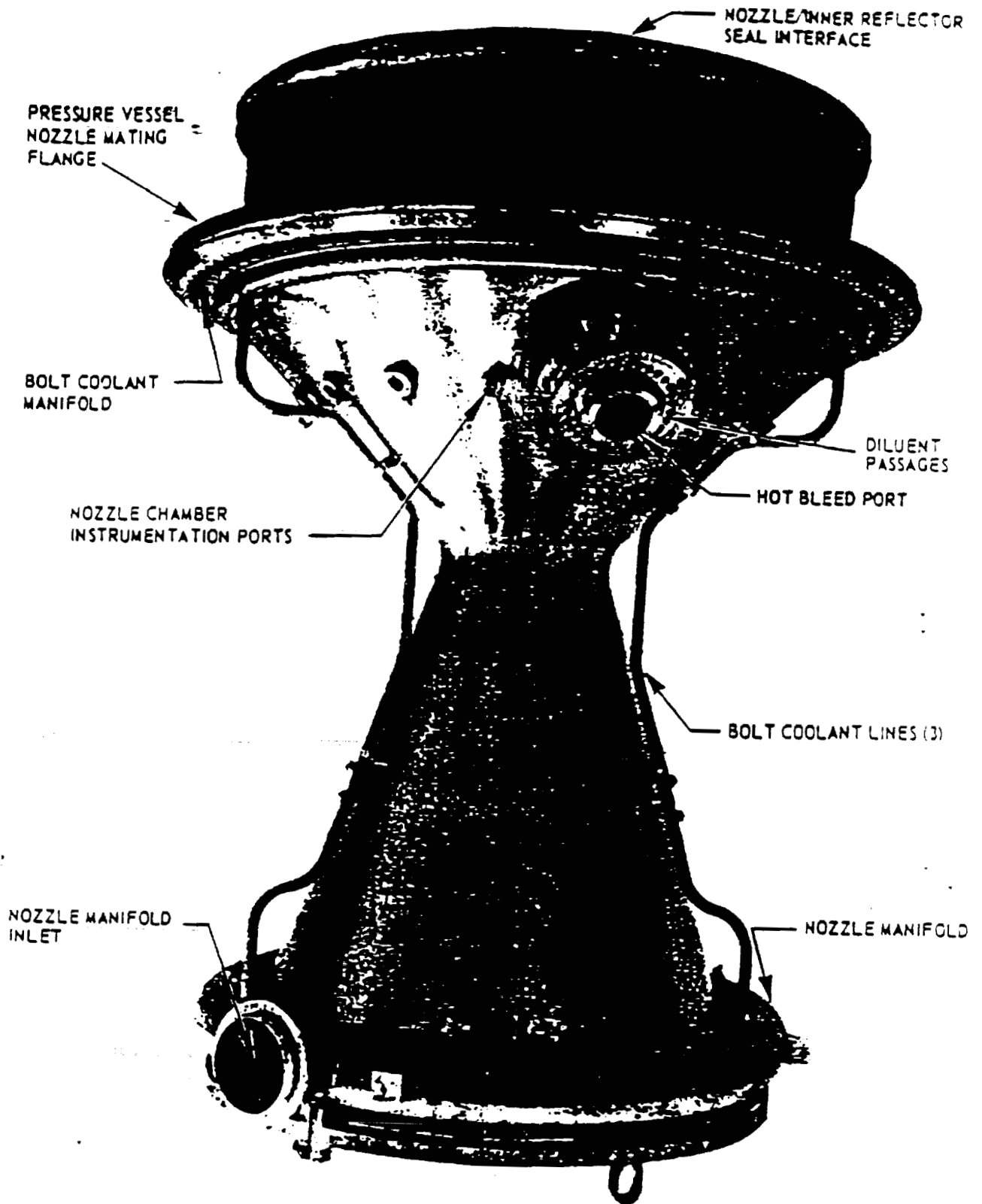
FIGURE 53. ENGINE NOZZLE.
