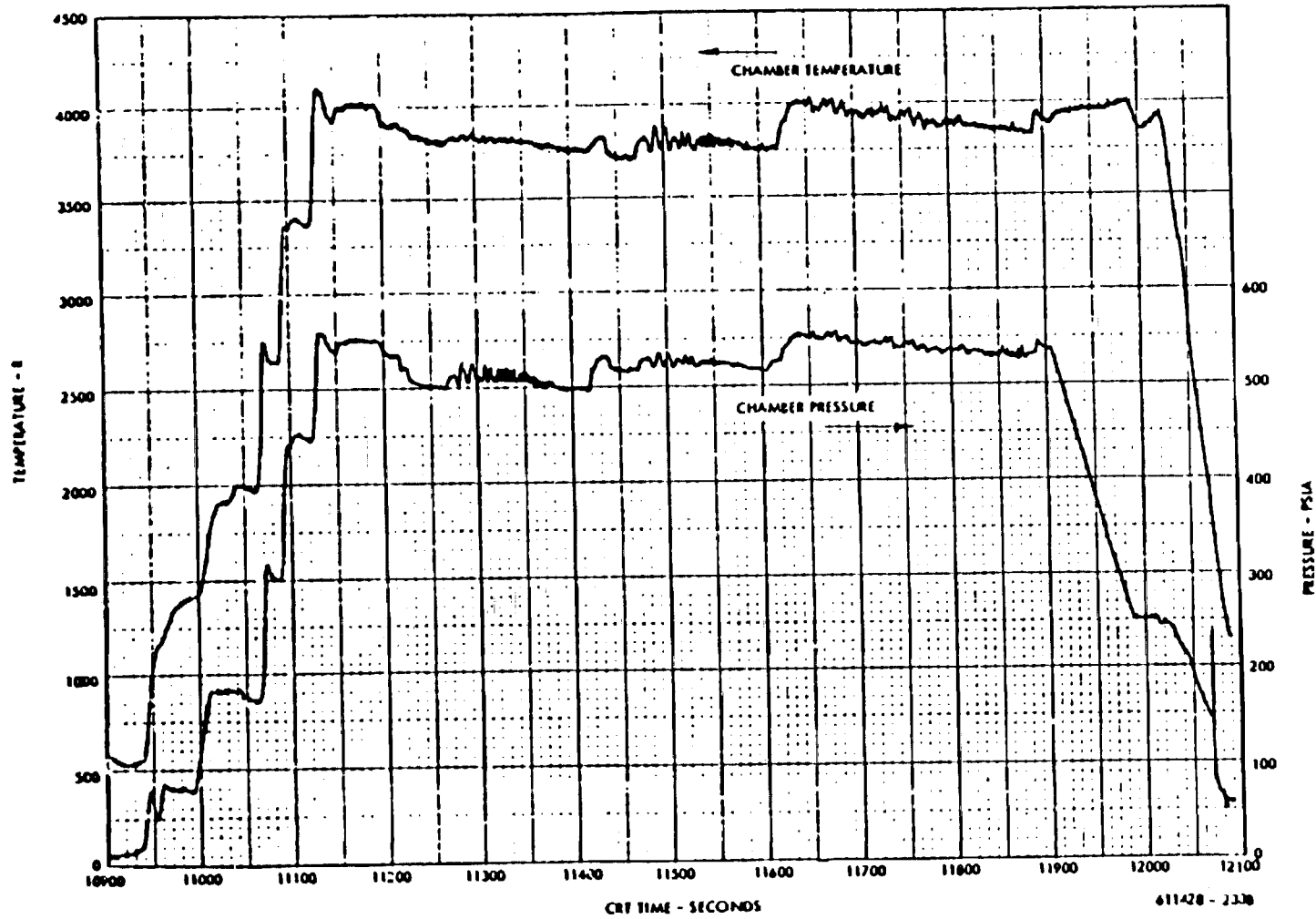
NRX/EST EP-IV, Profile (Sheet 1) - Full Power Endurance Test
