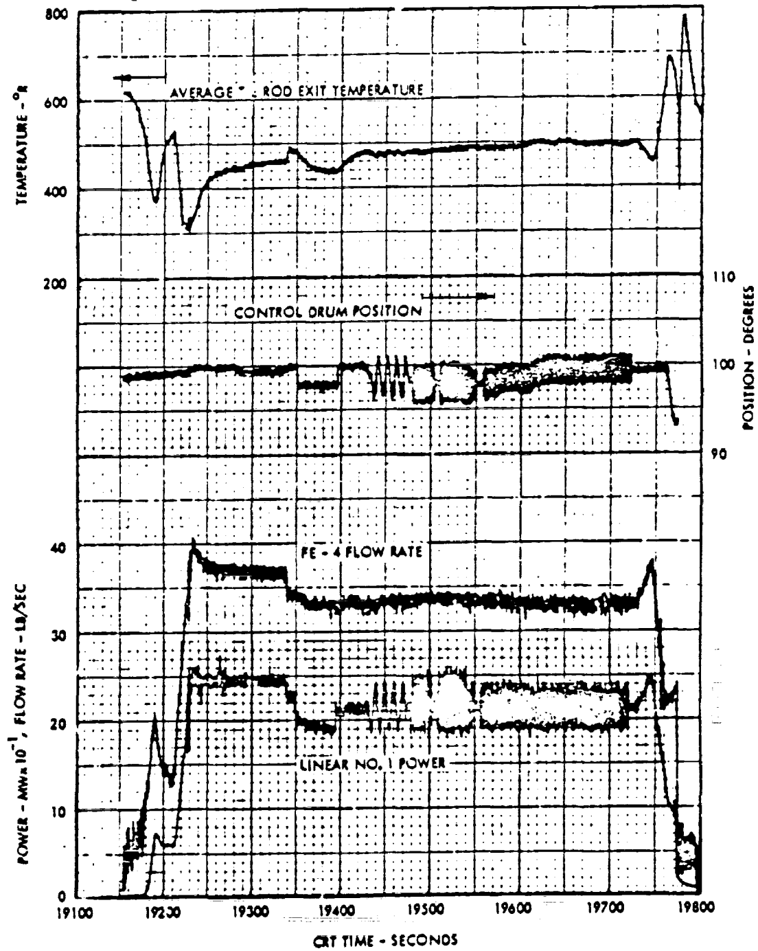
NRX/EST EP-IIC, Run 1 Profile (Sheet 2) - Complete Run
