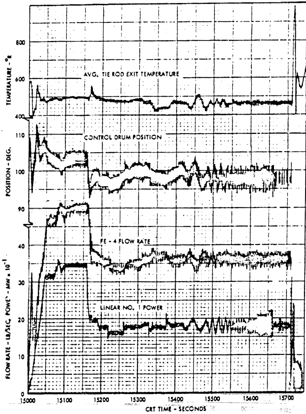
NRX/EST EP-IIB, Run 1 Profile (Sheet 2) - Complete Run
