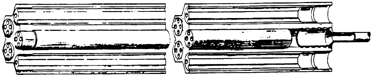
FIGURE 12. KIWI A' GRAPHITE MODULE-FUEL ELEMENT ASSEMBLY.
