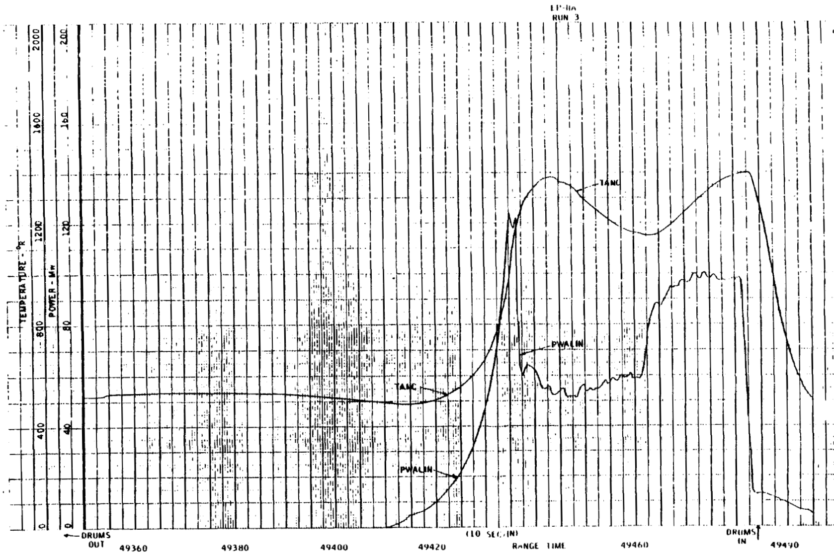
EP-2A Chamber Temperature and Power Vs Time (Sheet 2 of 2)
