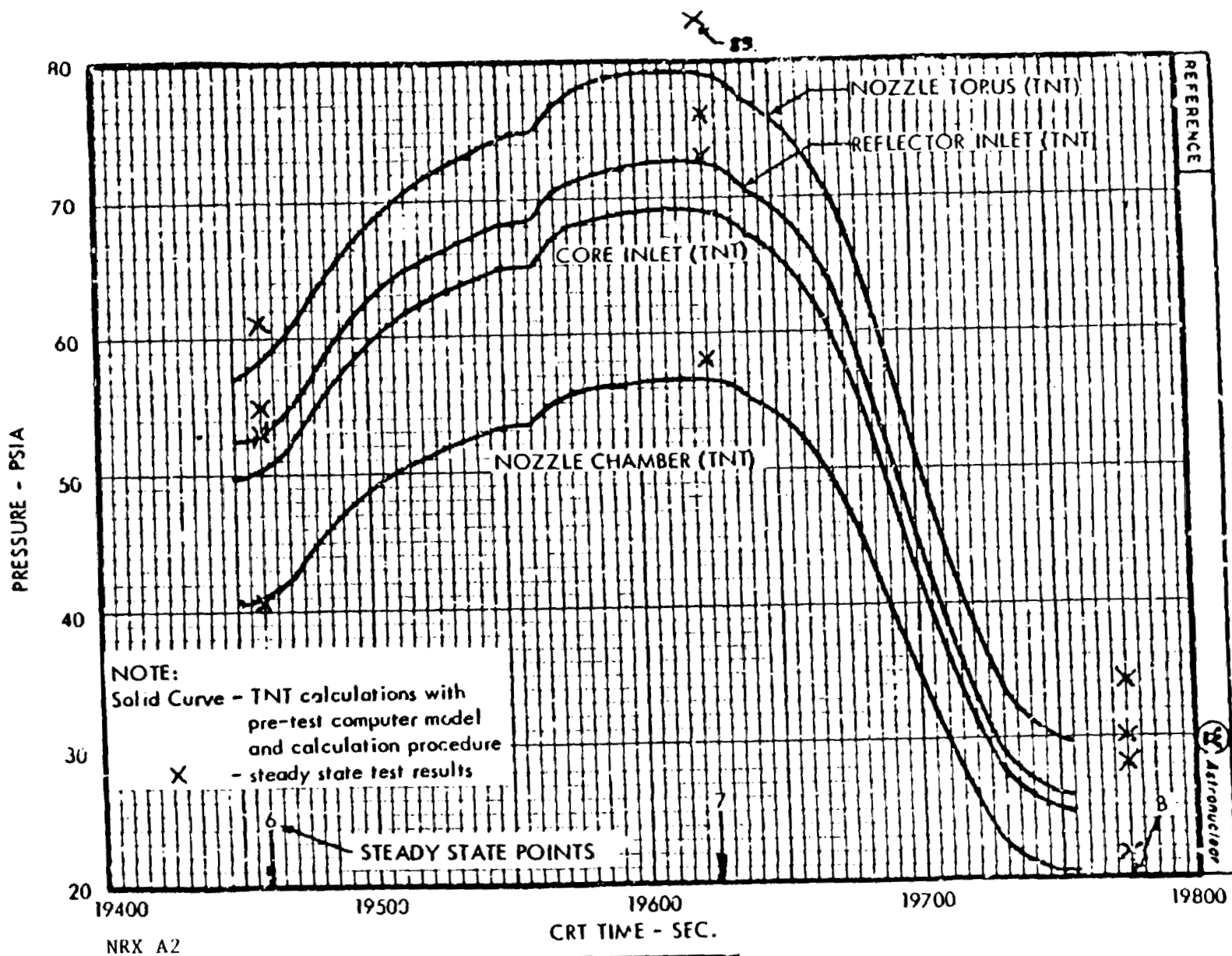
EP-V LOW POWER MAPPING TEST: FIXED CONTROL DRUMS REACTOR PLENUM PRESSURES
