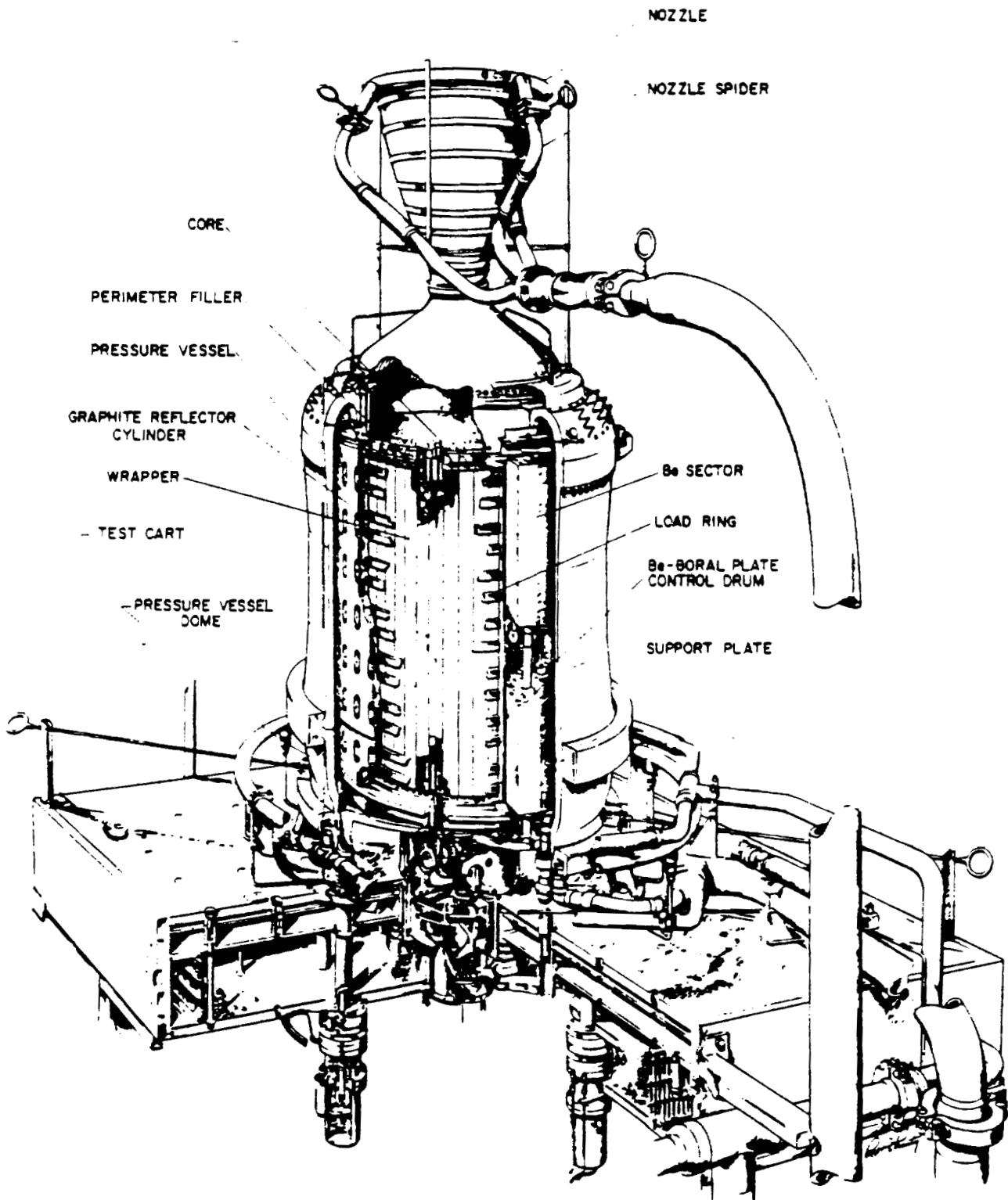
FIGURE 26. CUTAWAY VIEW OF KIWI B4D.
