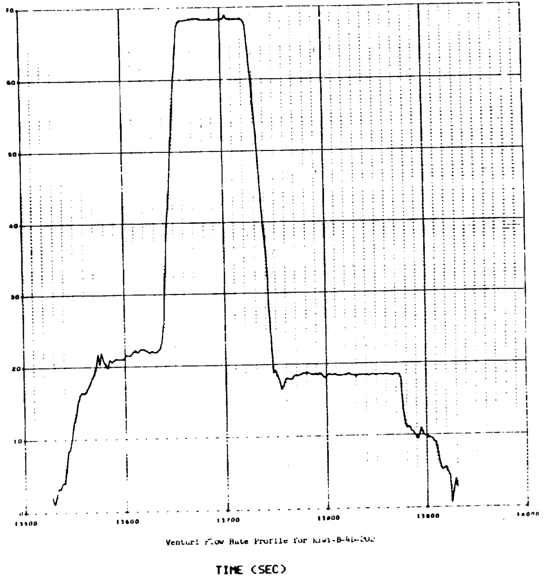
KIWI B4D LH2 Flow Rate Profile
