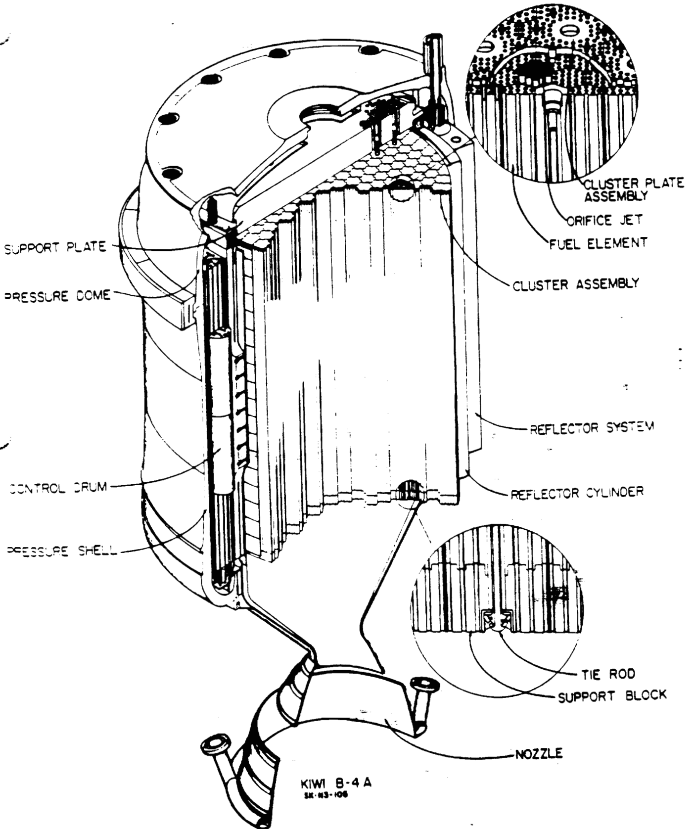
FIGURE 23. KIWI B4A REACTOR ASSEMBLY CUTAWAY.
