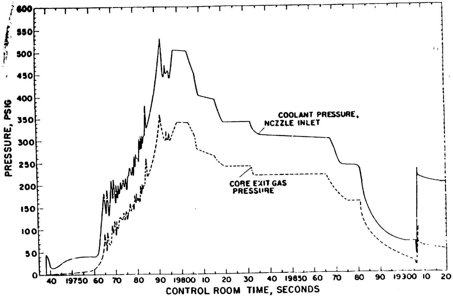
KIWI BIB Full-Power Run -- Nozzle Coolant Inlet and Core Exit Gas Pressures.
