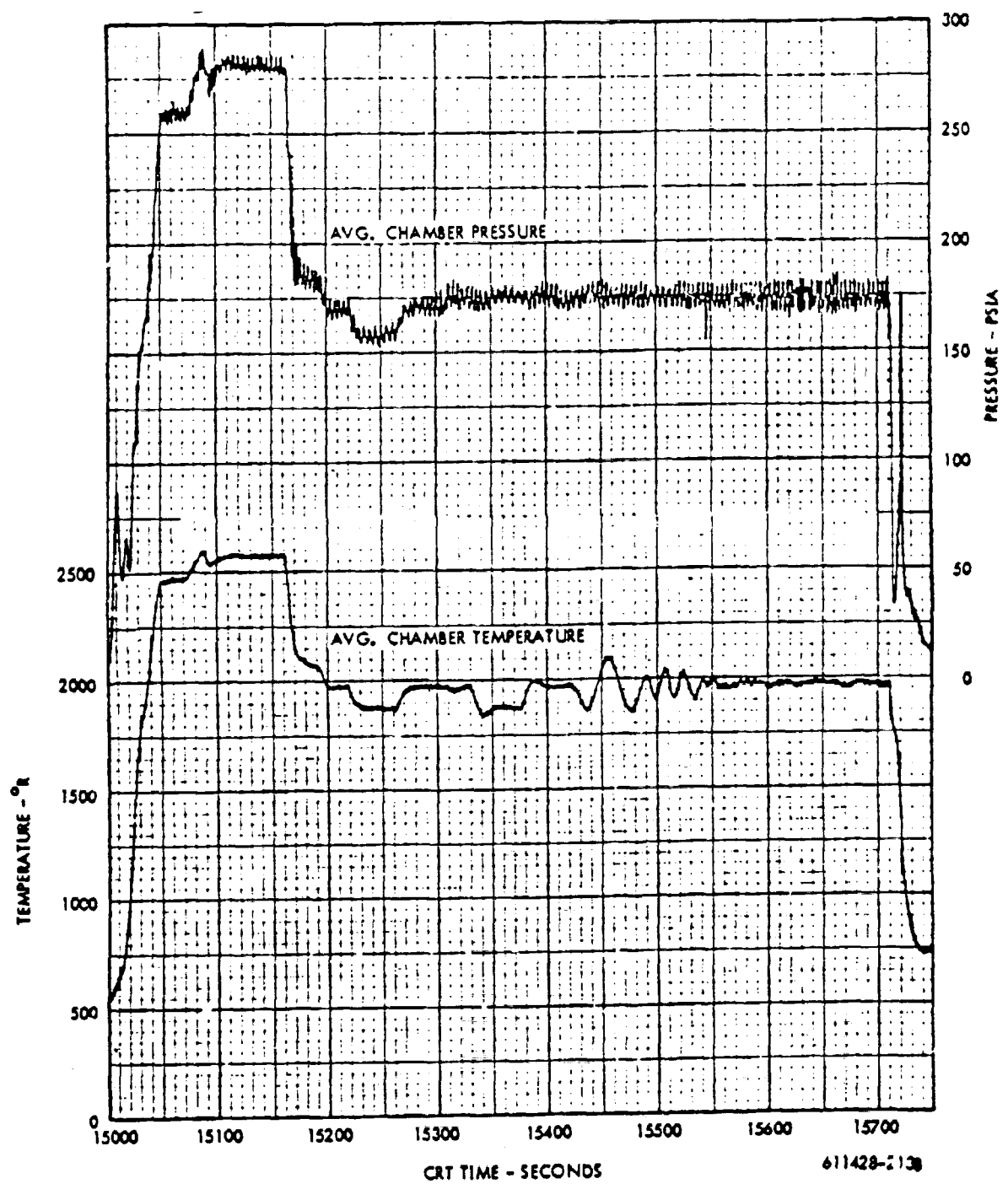
NRX/EST EP-IIB, Run 1 Profile (Sheet 1) - Complete Run
