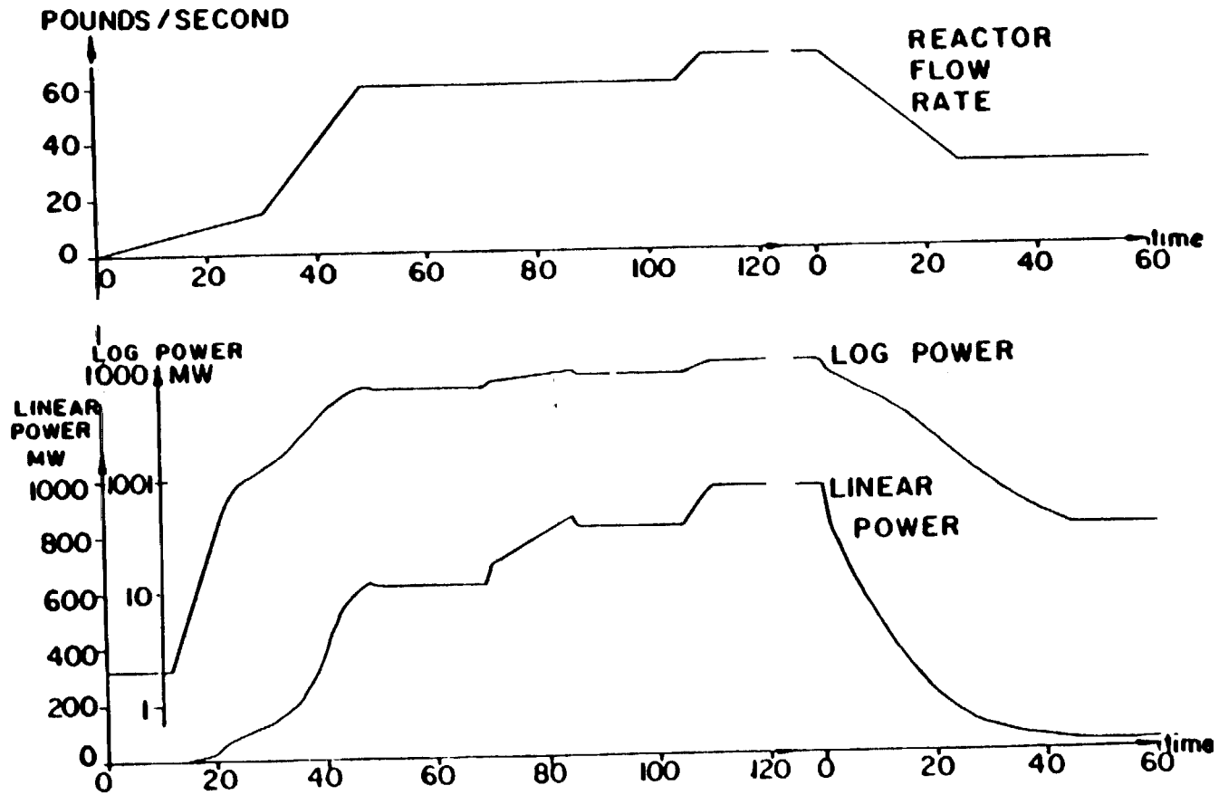
KIWI B4E Planned Flow Rate and Power Profiles
