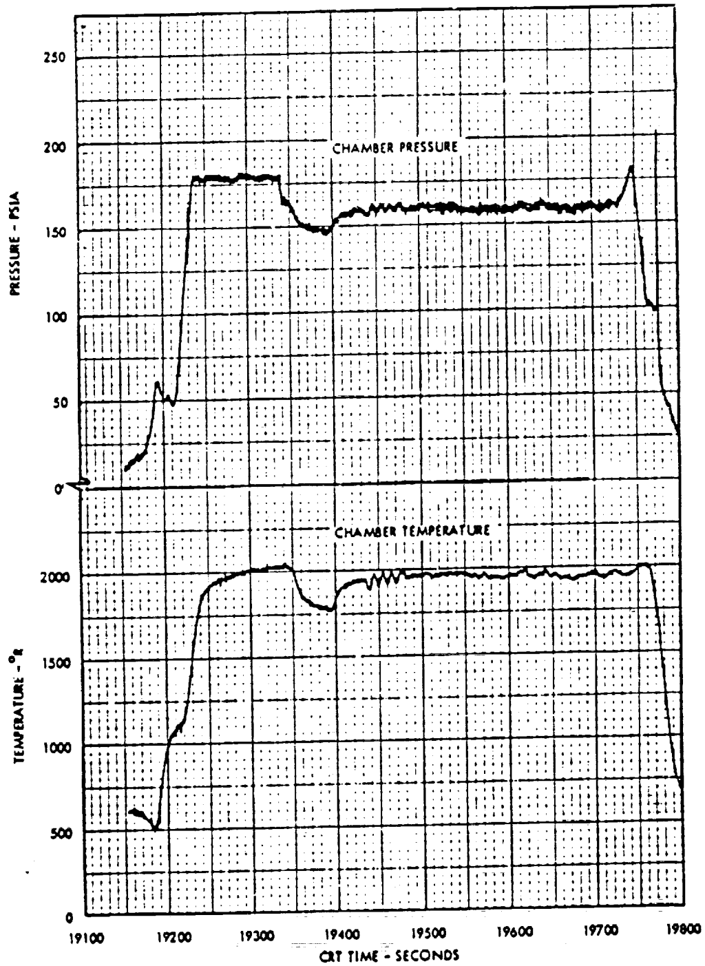
NRX/EST. EP-IIC, Run 1 Profile (Sheet 1) - Complete Run
