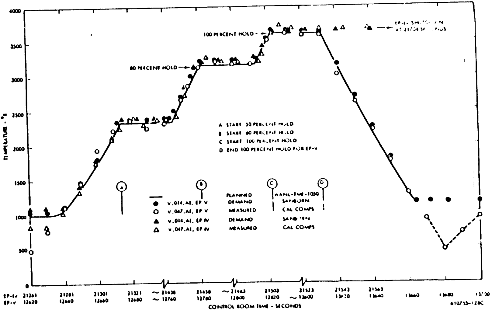
NRX-A3 Station 26 Temperature Programmer
