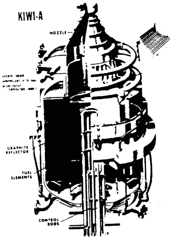
FIGURE 5. SECTIONED VIEW OF THE KIWI A.
