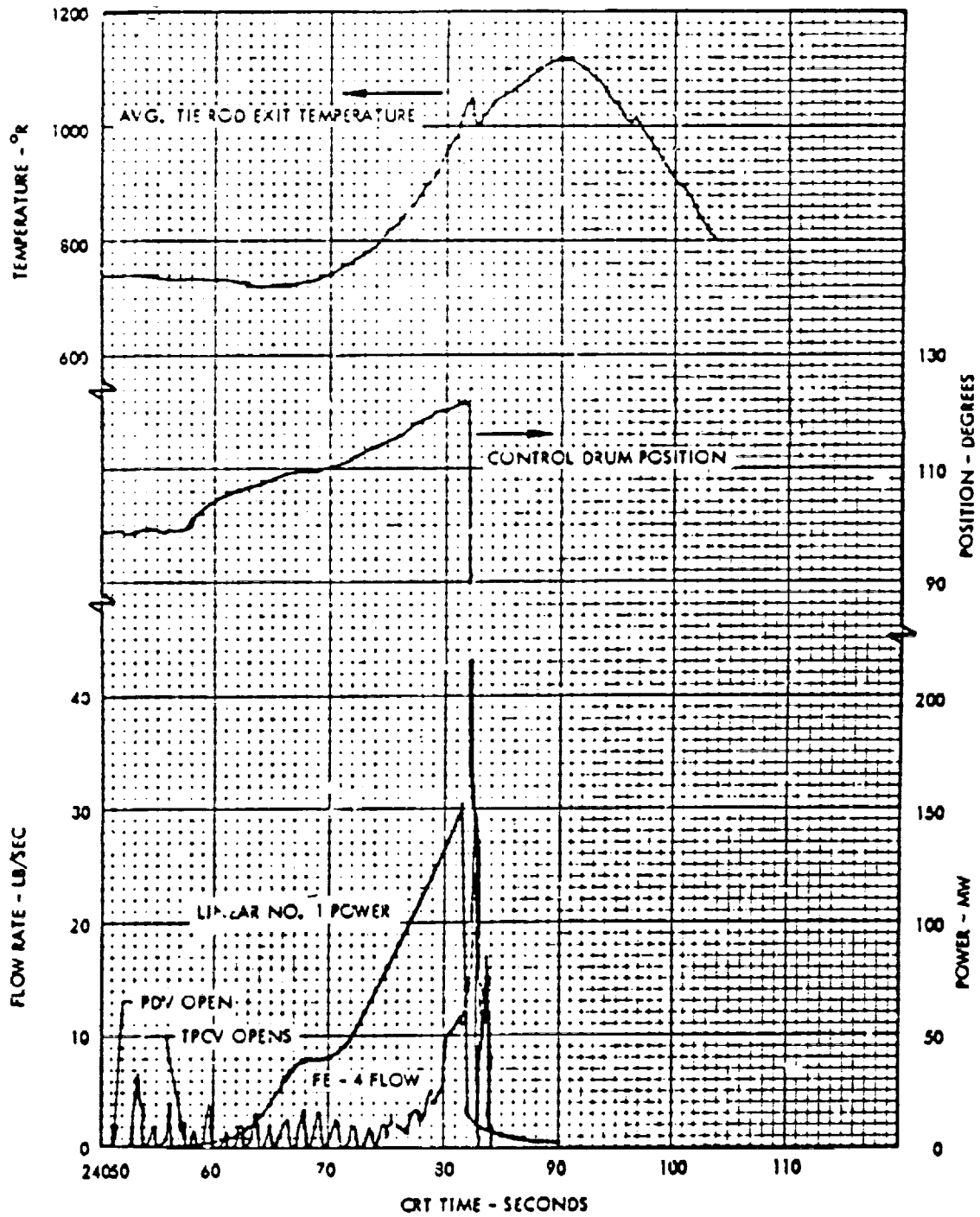
NRX/EST EP-II-C, Abort Run Profile (Sheet 2) - Low Dewar Pressure Bootstrap
