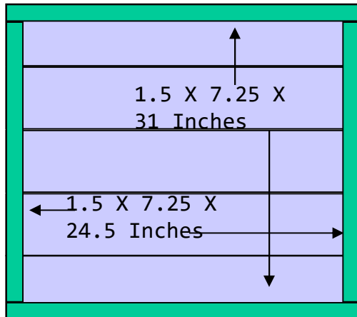
Top View of Bottom Frame
