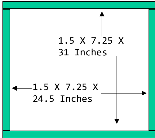
Top View of Top Frame
