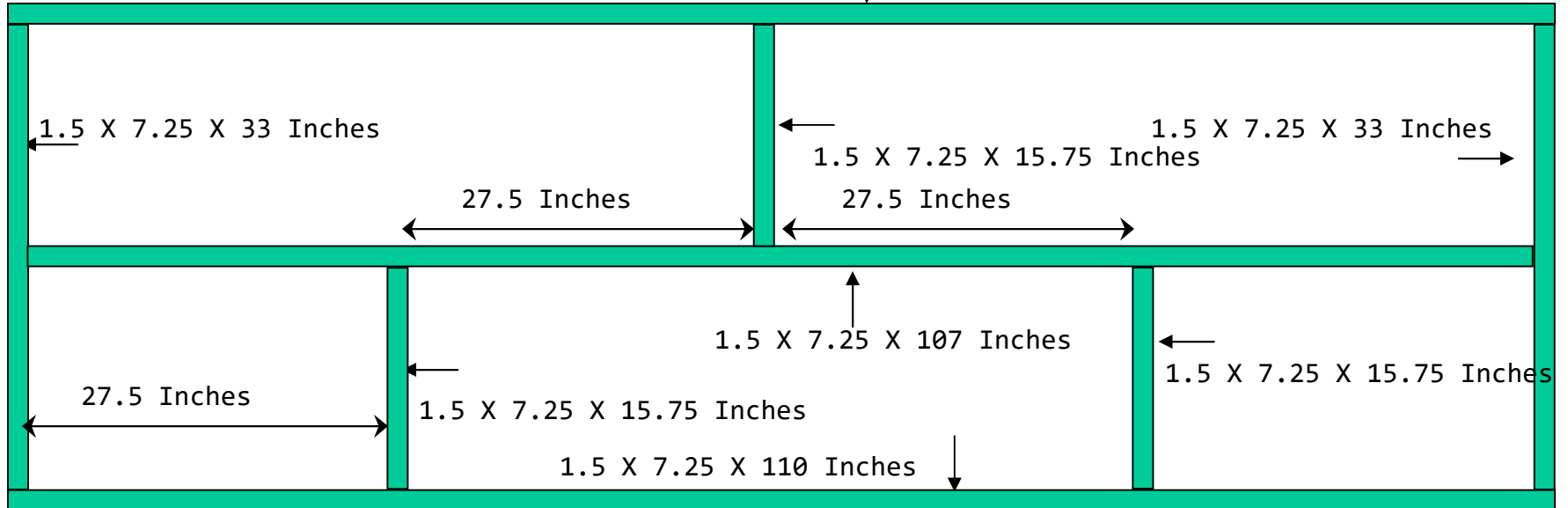
Top View of Bottom Frame
